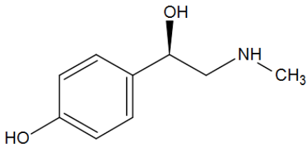
R -(-)-Synephrine
