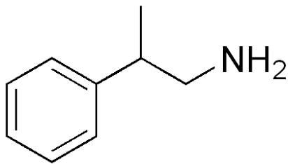
\beta -Methylphenethylamine
